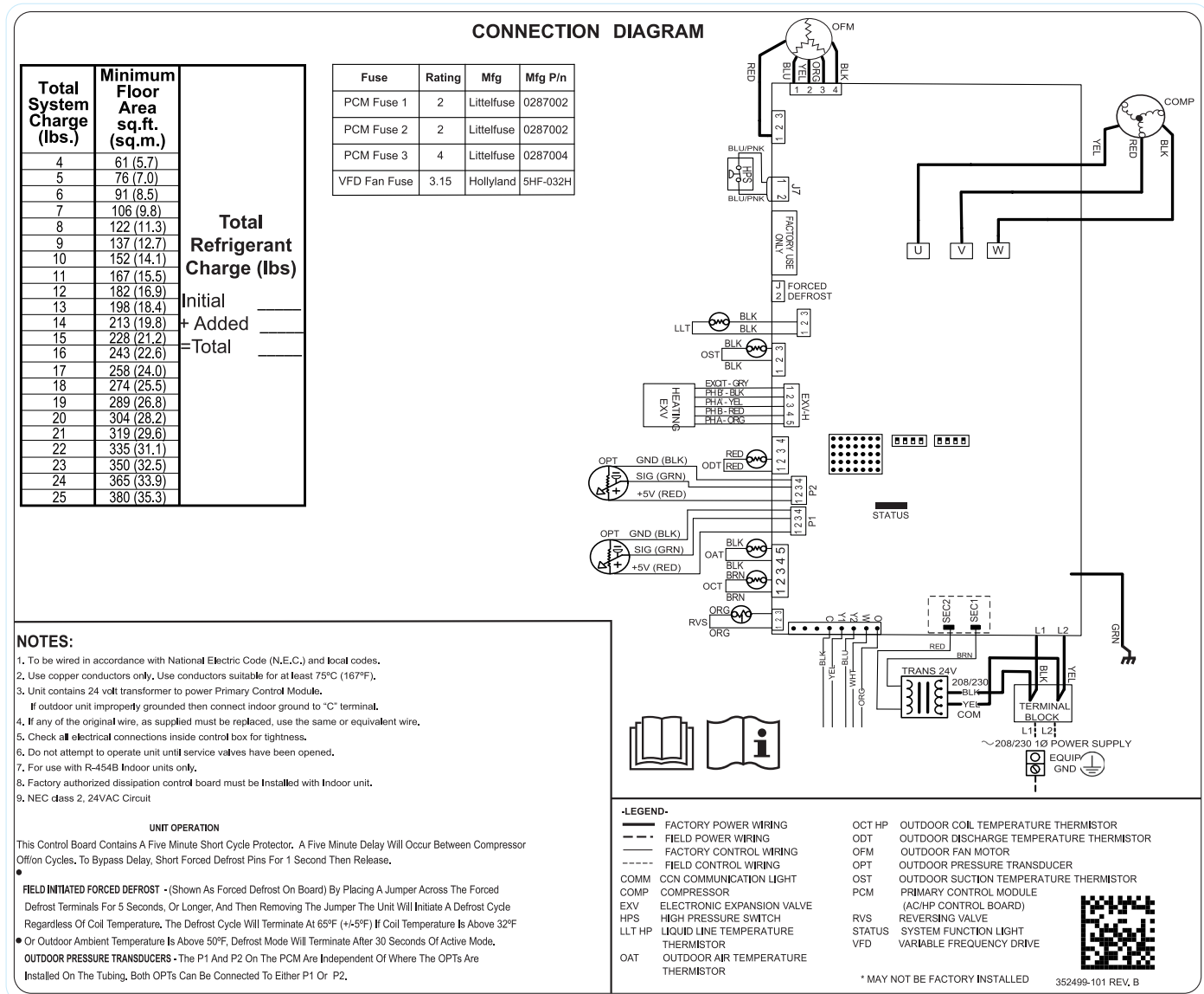
Fig. 1 – Size 2 - 5 Tons
