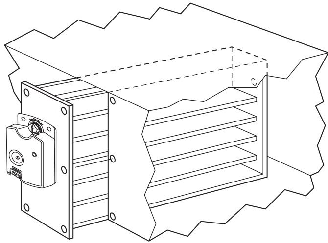
Fig. 3 – Slip-In Damper
