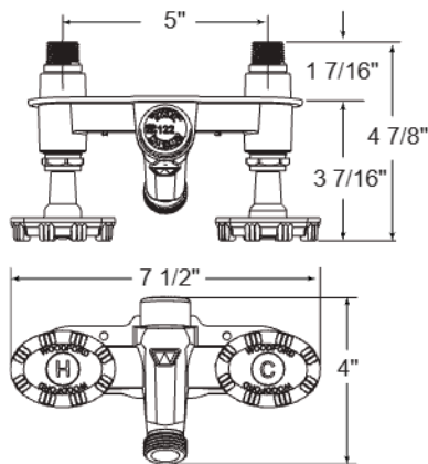
Model 122 Rough-In Dimensions
