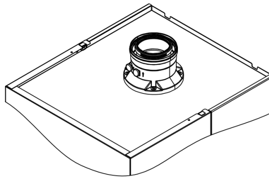
Vent Connection, models B2HA 112, 150, 399, 530
