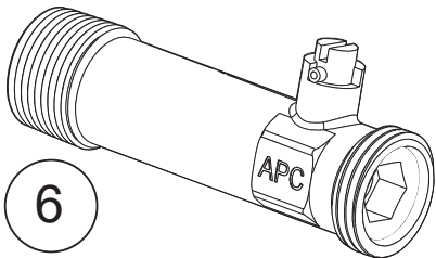
Figure 3. Drain Valve
