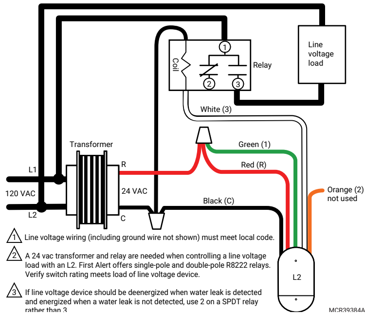
Fig. 13. L2 controlling a line voltage load.
