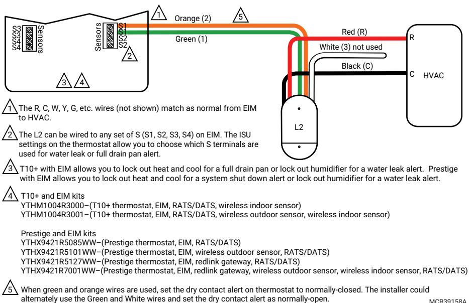
Fig. 9. L2 for water leak alert or full drain pan alert on T10+ with EIM or Prestige with EIM.
