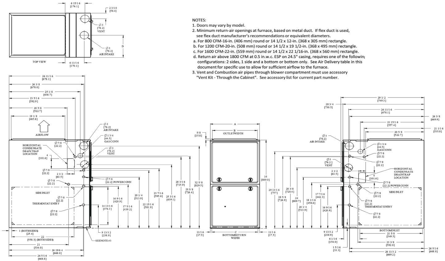
A210796 Dimensions
