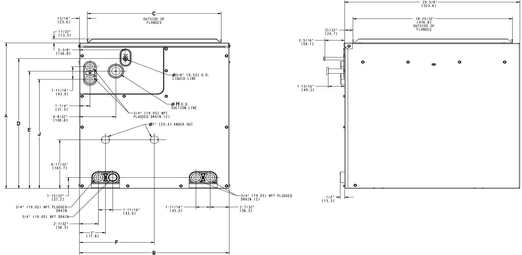
Fig. 9 – EVM5X Dimensions
