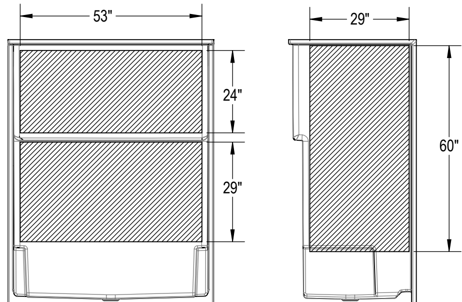
Full Wall Reinforcement Option
