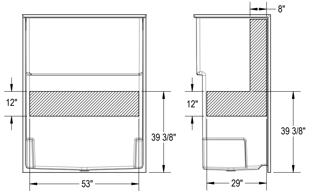
FHA Reinforcement Option
