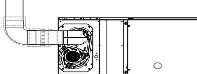
Downflow Application-Vent Elbow Left then Up
