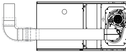
Upflow Application-Vent Elbow Right
