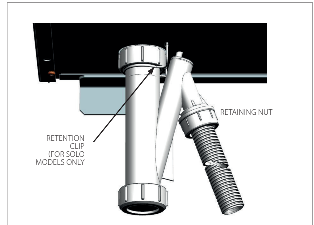
Fig. 2 - Condensate Retention Clip - (Solo Models only)
