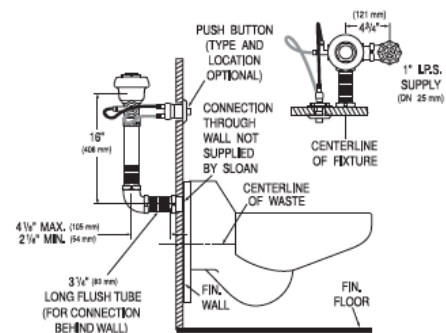
Combination Fixture
