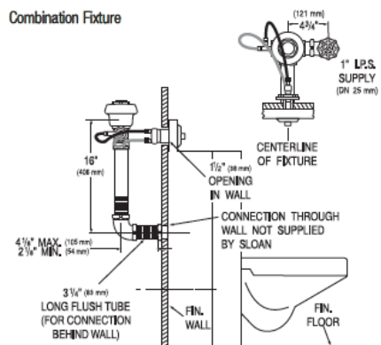
Combination Fixture
